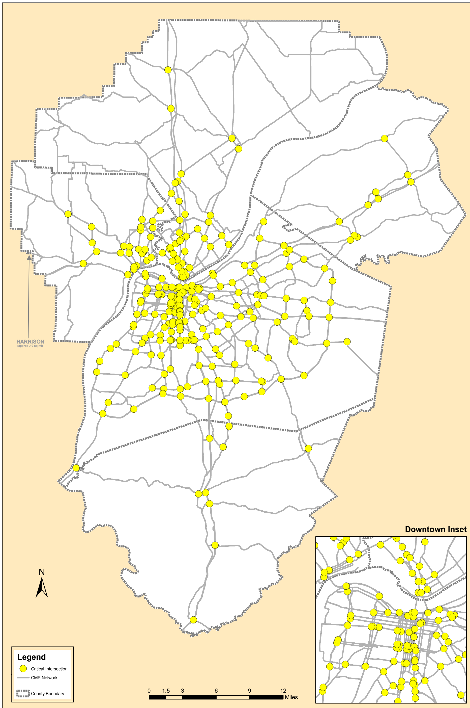
FIGURE 7 LOUISVILLE (KY-IN) MPA CONGESTION MANAGEMENT PROCESS ROADWAY NETWORK CRITICAL INTERSECTIONS
